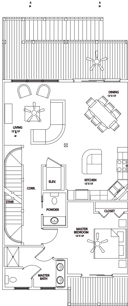
LEVEL 2 LIVING LEVEL FLOOR PLAN 1/4" = 1'-0"
