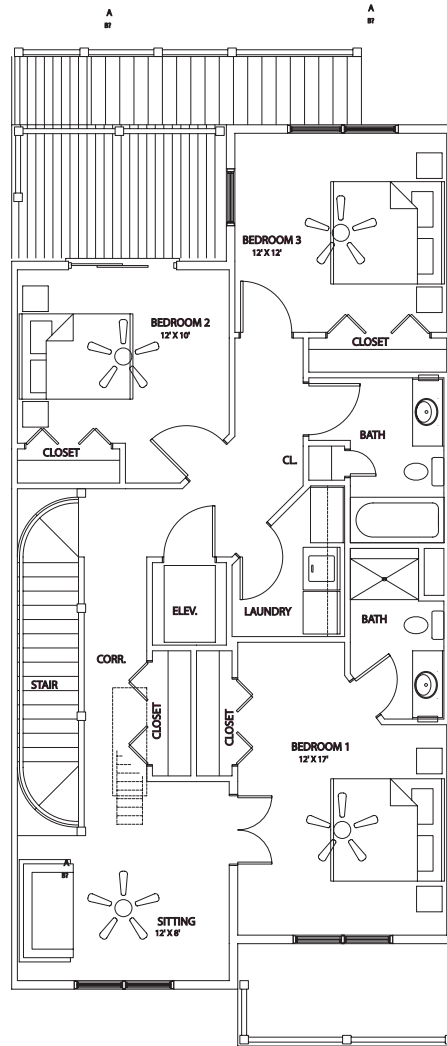
LEVEL 3 SLEEPING LEVEL FLOOR PLAN 1/4" = 1'-0"
